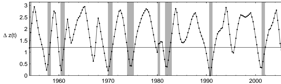
FIGURE 4.— Differences \Delta z(t) between the instantaneous-phase vector \phi(t) and its value at the reference time t_{\text{ref}} = 1990:3 ; see (10). The shaded areas indicate NBER dates of U.S. recessions, as in Fig. 1, while the horizontal line placed at \Delta z(t) = 1.2 indicates our threshold for selecting the minima of \Delta z(t) .
