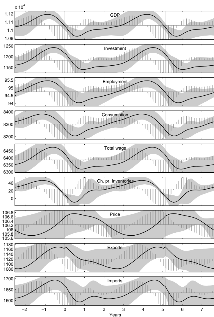
FIGURE 5.— The average business cycle, with the cycle length set to 5.2 years. Heavy solid lines show the average over the individual cycles, while the gray areas indicate the corresponding standard deviation, and the shorter vertical lines indicate the one-year growth rate. For better visualization, about half the cycle is repeated on either side of the full period.
