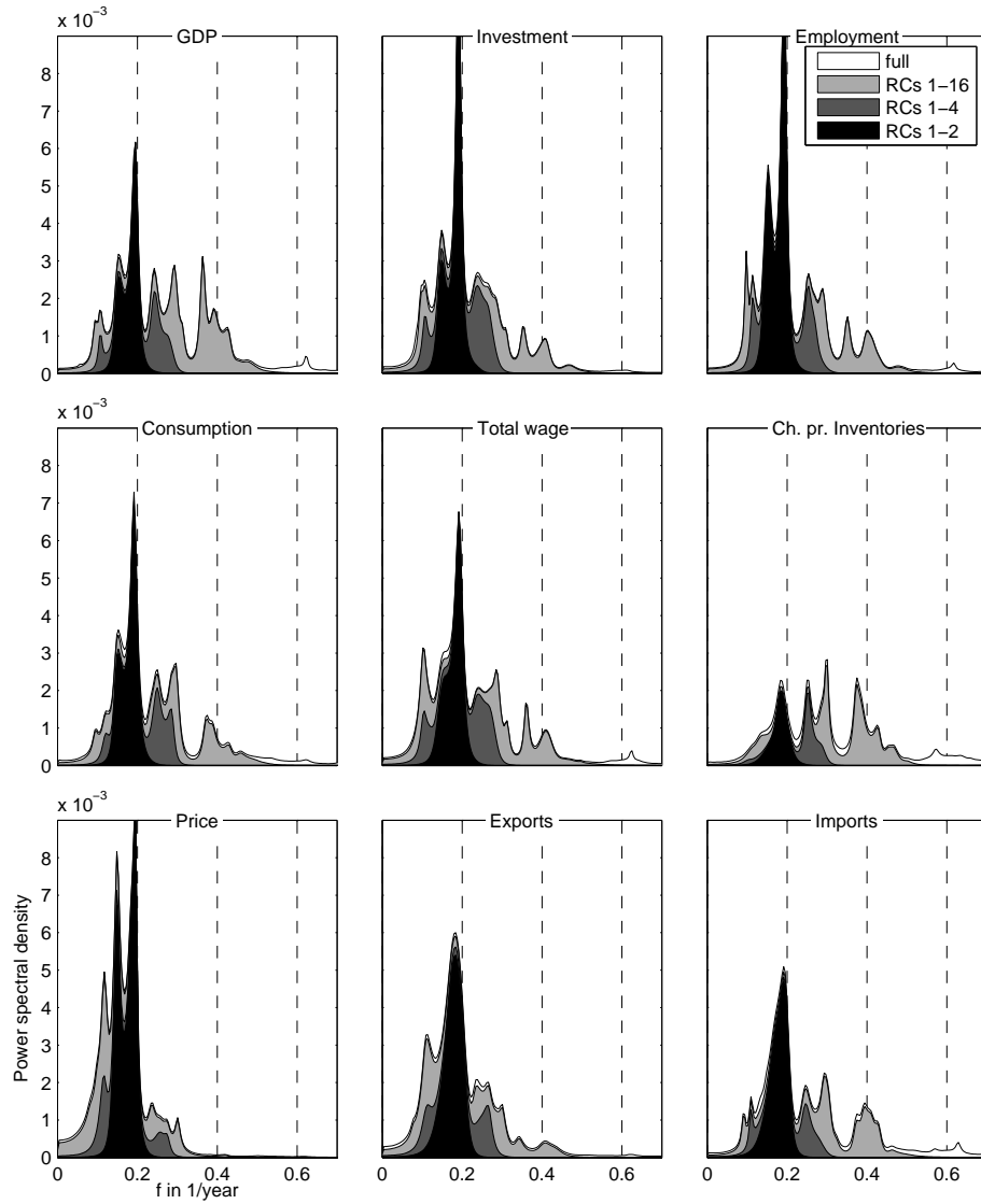
FIGURE 3.— Successive reconstruction of the spectral densities of the nine U.S. macroeconomic indicators. The different shadings (see legend in upper-right corner) indicate the “stacking” — i.e., the separate contributions — of the power spectra of different subsets of reconstructed components (RCs). The 5.2-year peak captured by RCs 1-2 clearly dominates all the economic indicators.
